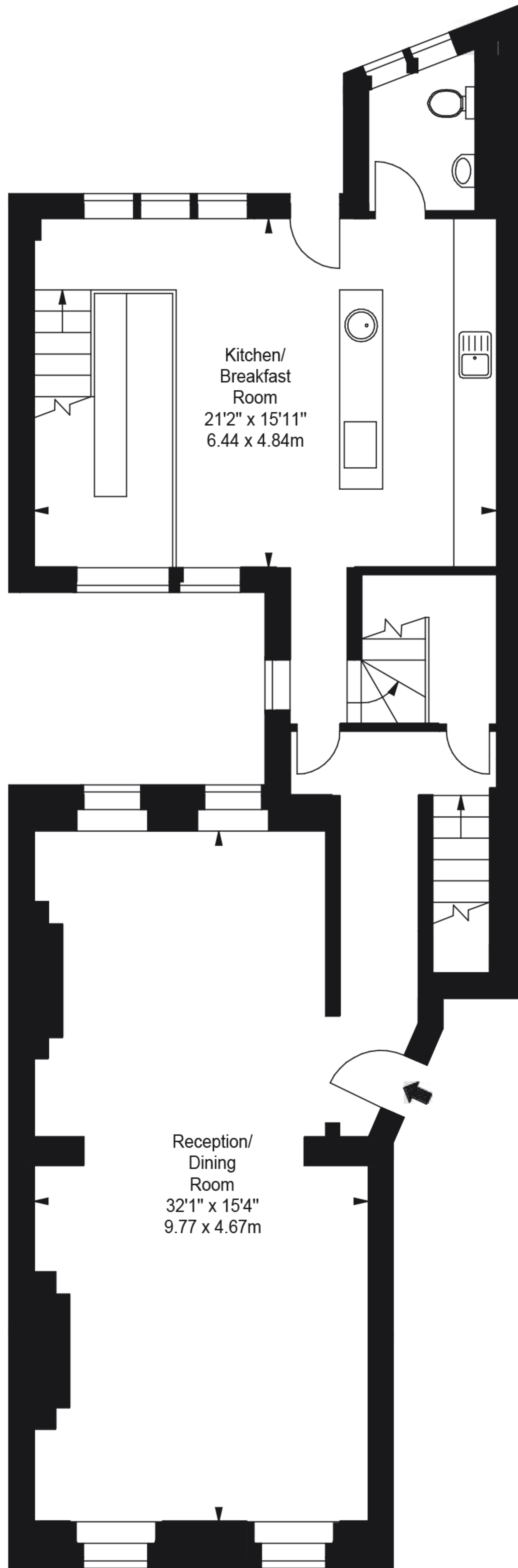
Ground Floor
