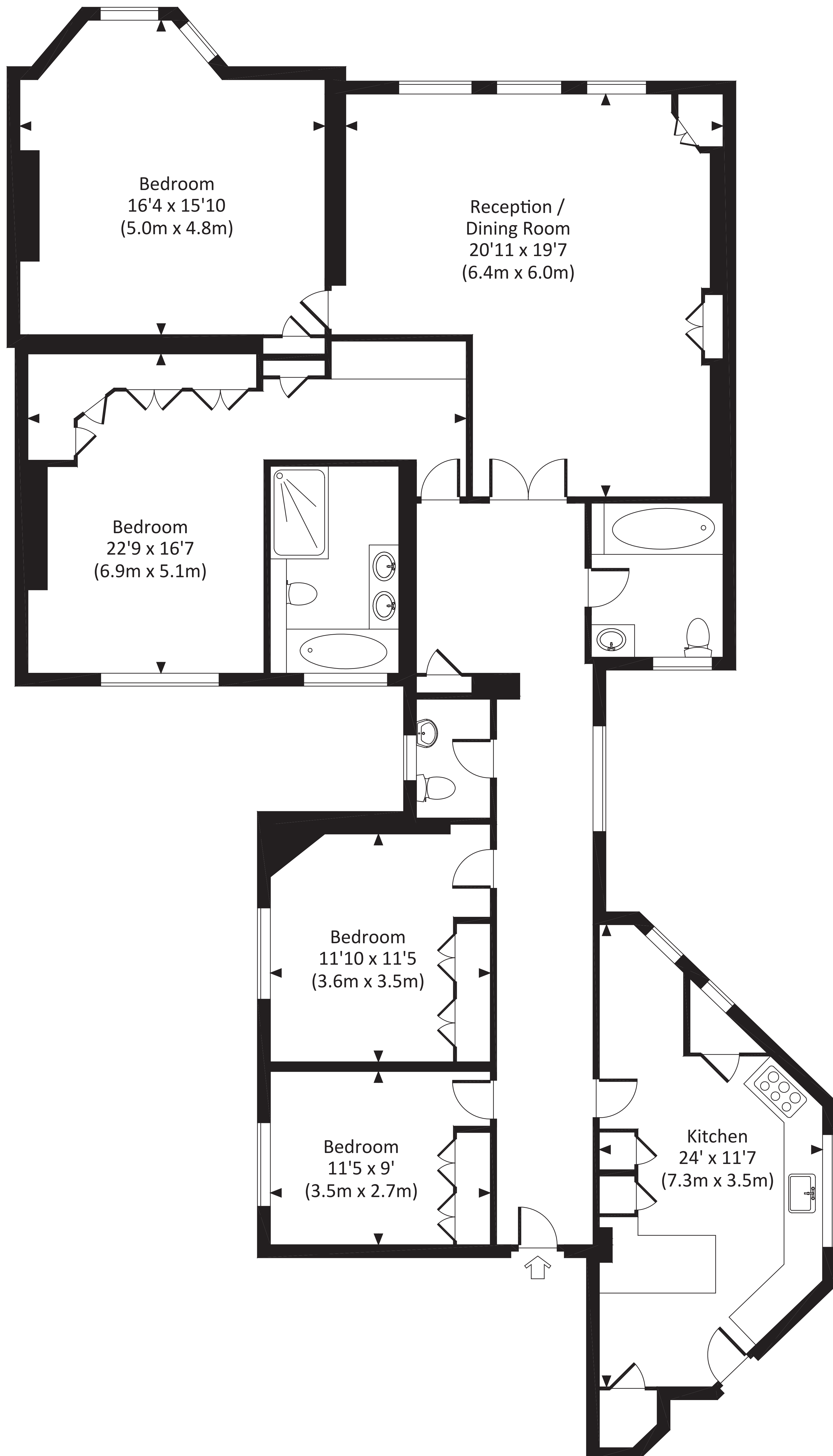
SECOND FLOOR
